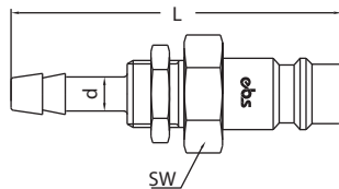
Panel Hortum Uç / Panel Mount Plastic Hose Plug
