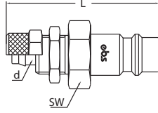
Plastik Hortum Uç / Plastic Hose Plug
