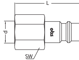
Panel Hortum Uç / Panel Mount Plastic Hose Plug
