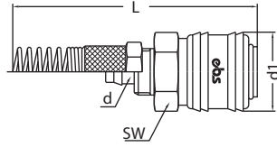
Yaylı Plastik Hortum Gövde / Plastic Hose Coupling with Spring
