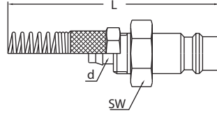
Yaylı Plastik Hortum Uç / Plastic Hose Plug with Spring
